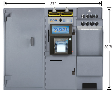
Tidel Series 4 with Standard Side Vault and Tube Vend
