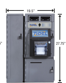
Tidel Series 4 with Narrow Side Vault
